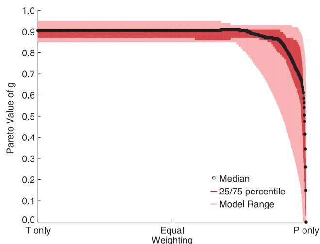
Figure 3. The maximum amount of geoengineering ( g ) as determined by the Pareto criterion (7) as a function of the relative weighting ( w ) between temperature and precipitation. Values shown represent the median, quartiles, and range of the 12 models included in this study.
